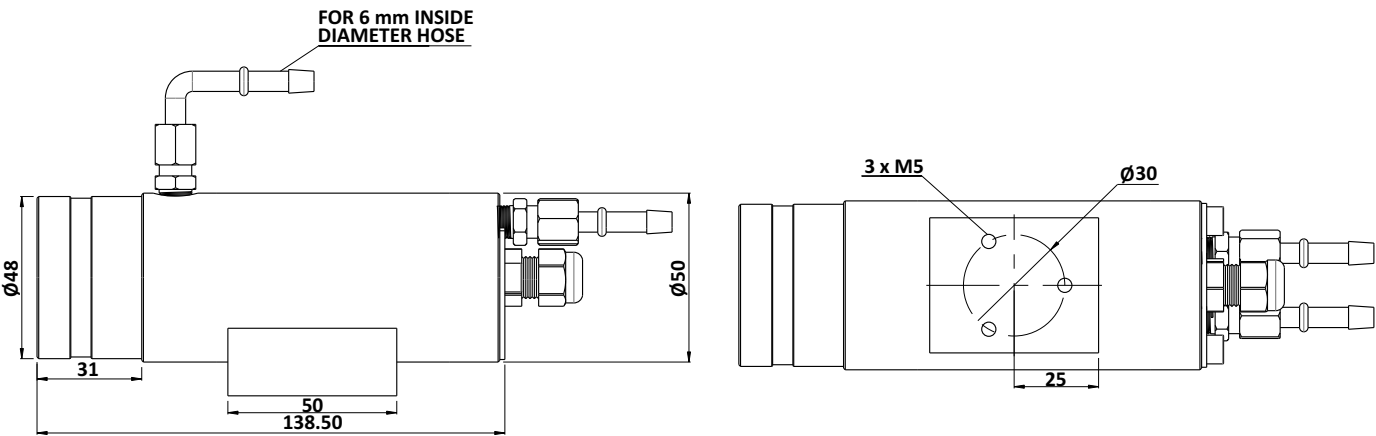
Water Cooling Jacket with Adjustable Flange PL (Reference no: 8000-02)
