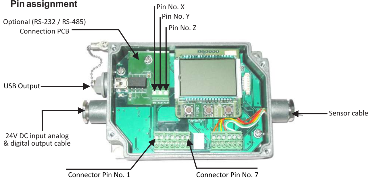
Fig. 5 Pin Assignment
