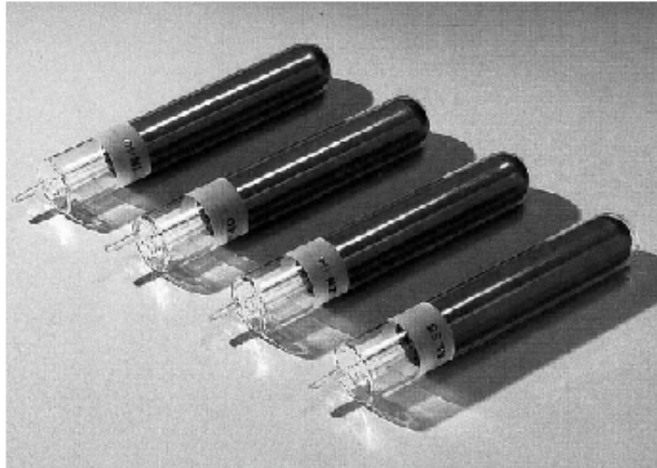
Figure 1. Triple point of water cell
