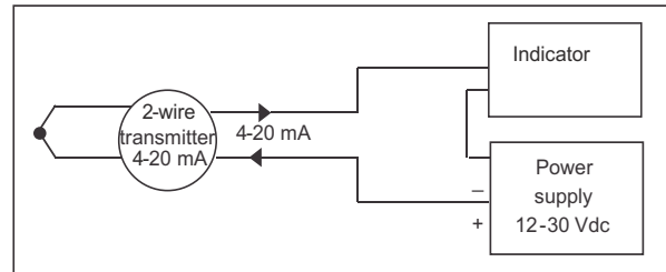
Temperature Transmitter 2- wire
