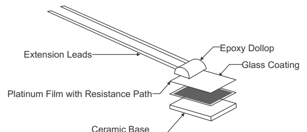
Platinum thin film RTD
